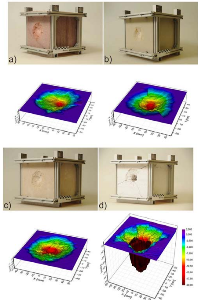
Figure 1. Examples of the results of gas-gun experiments on asteroid surface analog materials carried out by NEOShield partner Fraunhofer Ernst Mach Institute, Freiburg, Germany. The impact craters in different target materials with porosities, \phi , were formed by projectiles with approximately the same impact velocity: a. Quartzite ( \phi \sim 3\% ); b. sandstone ( \phi \sim 25\% ); c. limestone ( \phi \sim 31\% ); d. aerated concrete ( \phi \sim 87\% ). In each case a photograph of the target after the impact is shown above a three-dimensional model of the crater morphology. The colour code shown adjacent to the bottom right crater model applies to all four models. The experiments demonstrate that large craters are formed in highly porous material but in contrast, the ejected mass is small. © Fraunhofer EMI.
