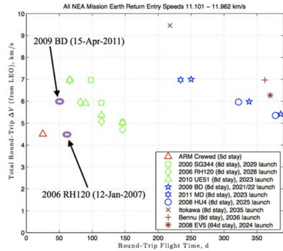
Figure 2: Comparison of round-trip mission accessibility for selected NHATS-compliant NEAs and an object in lunar DRO. Dates in parenthesis correspond to NEA mission Earth departure.
