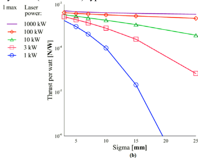
Figure 1. 2D analytic model results using SiO 2 as the equivalent material. (a) Integrated mass ejection rates vs. sigma case for different powers between 1 kW and 1 MW. (b) Similarly, integrated thrust (N) per watt vs. sigma.
